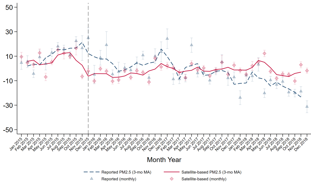
Figure 1: Reported and Satellite-based PM_{2.5} Trends
