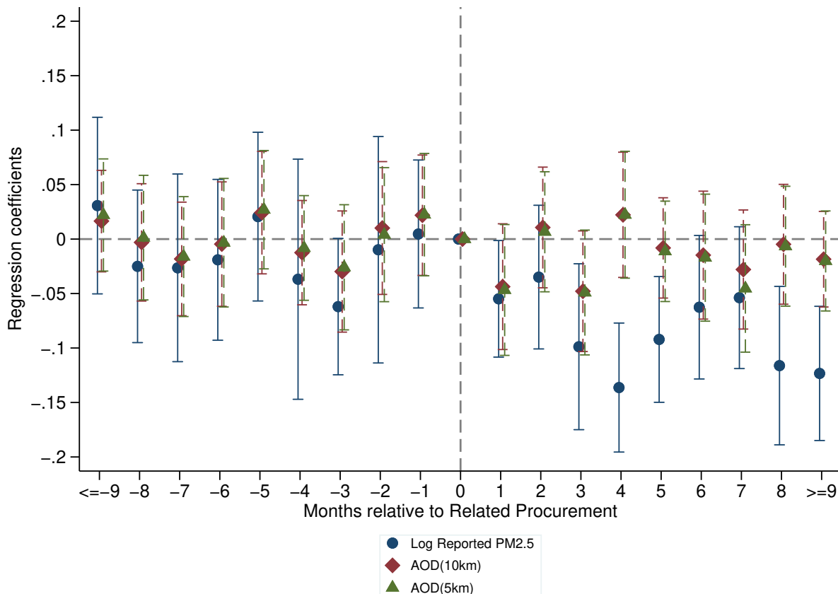
Appendix Figure A1: Dynamics of Reported PM_{2.5} versus AOD
